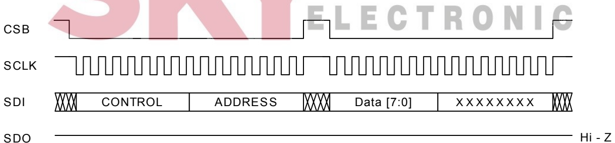
Figure 41. Write Operation via a 16-bit SPI Port
