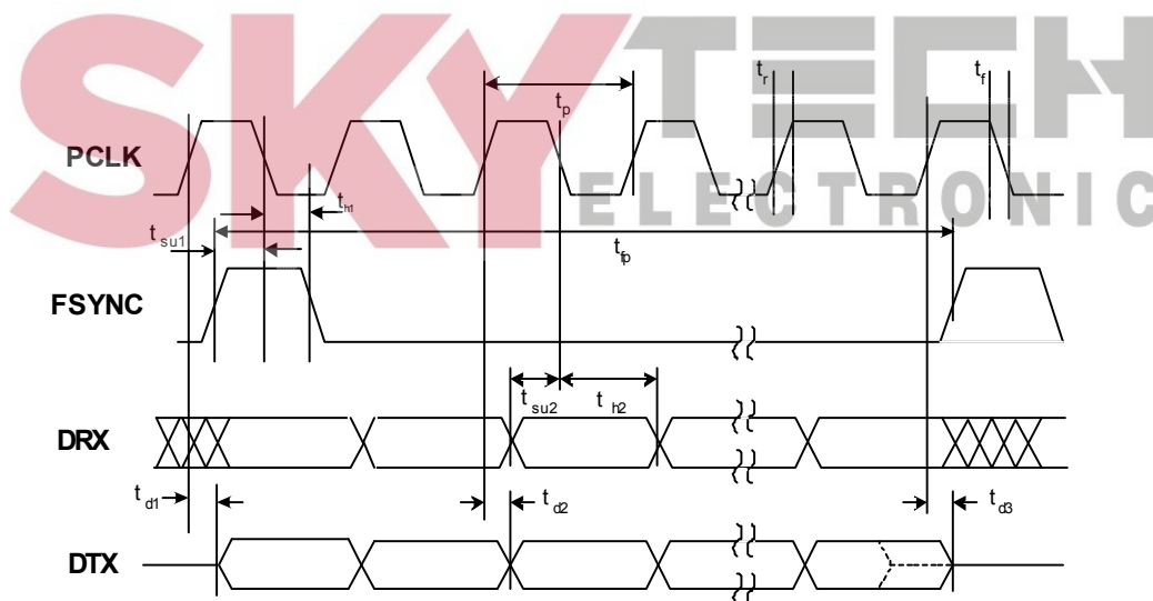
Figure 5. GCI Highway Interface Timing Diagram (1x PCLK Mode)
